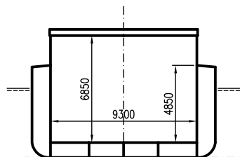
MIDSHIP SECTION
