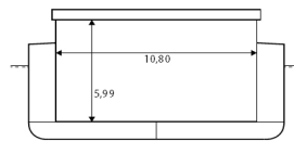
MIDSHIP SECTION
